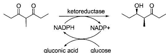
Figure 1. Enzymatic reduction of 4-methyl-3,5-heptanedione with NADPH-dependent ketoreductases.
