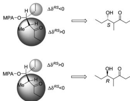
Figure 2. Determination of the stereochemistry of the hydroxy group of 5-hydroxy-4-methyl-3-heptanone.
