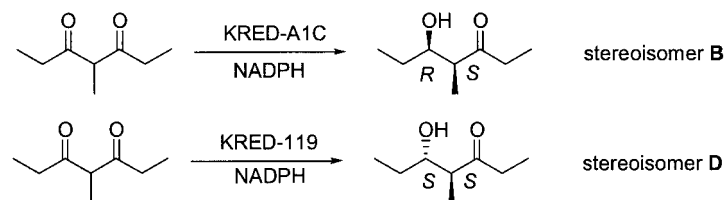
Figure 3. The absolute stereochemistry of the B, D stereoisomers of 5-hydroxy-4-methyl-3-heptanone.
